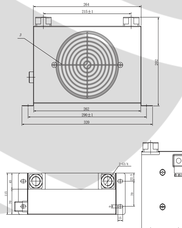
产品线图 PRODUCT LINE DIAGRAM
