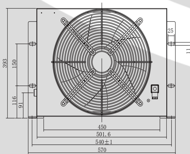
产品线图 PRODUCT LINE DIAGRAM
