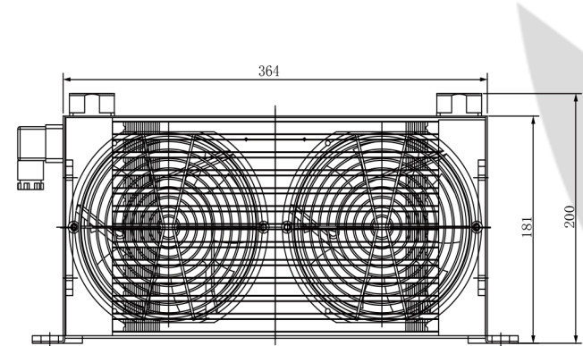
产品线图 PRODUCT LINE DIAGRAM
