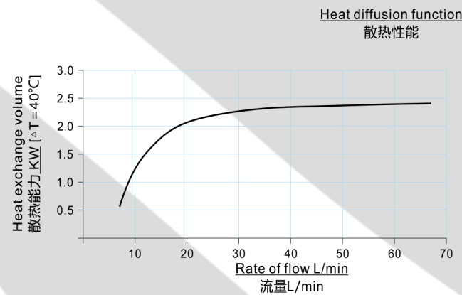
性能曲线 PERFORMANCE CURVE
