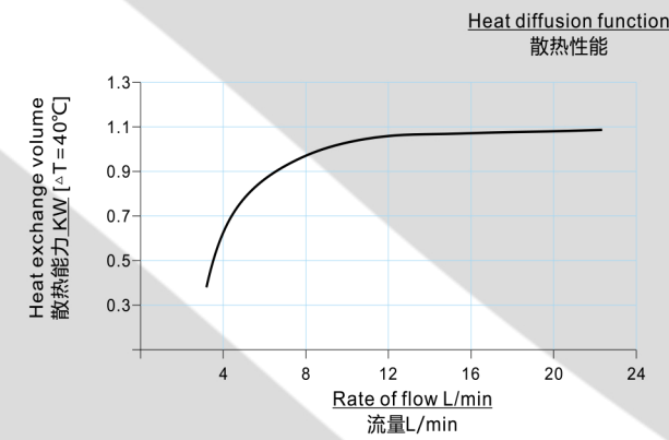
性能曲线 PERFORMANCE CURVE
