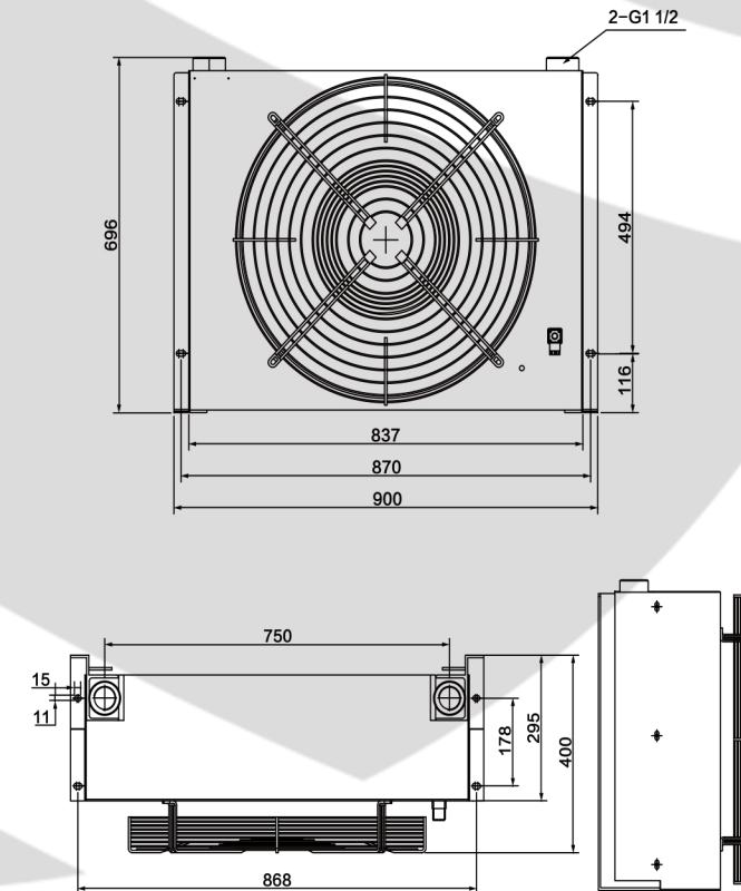
产品线图 PRODUCT LINE DIAGRAM
